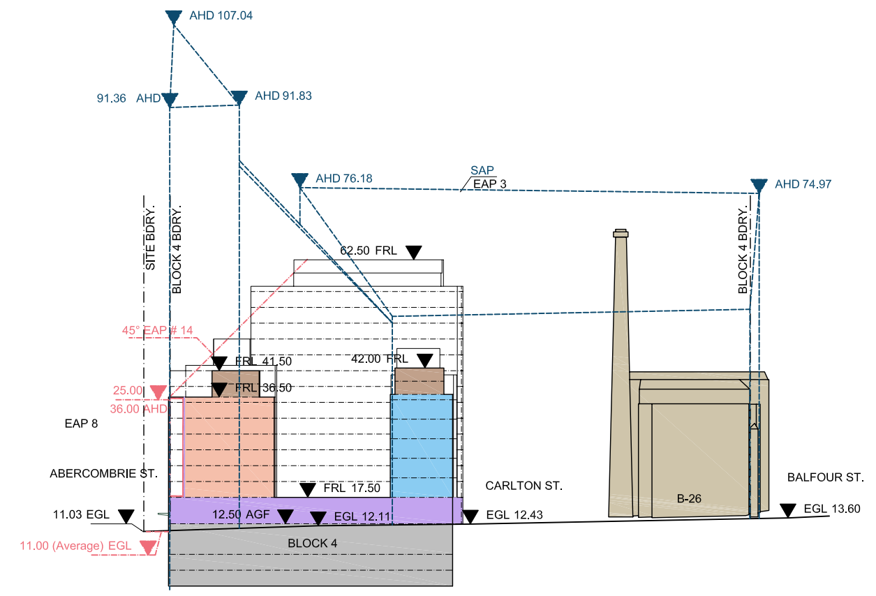
SECTION CC
