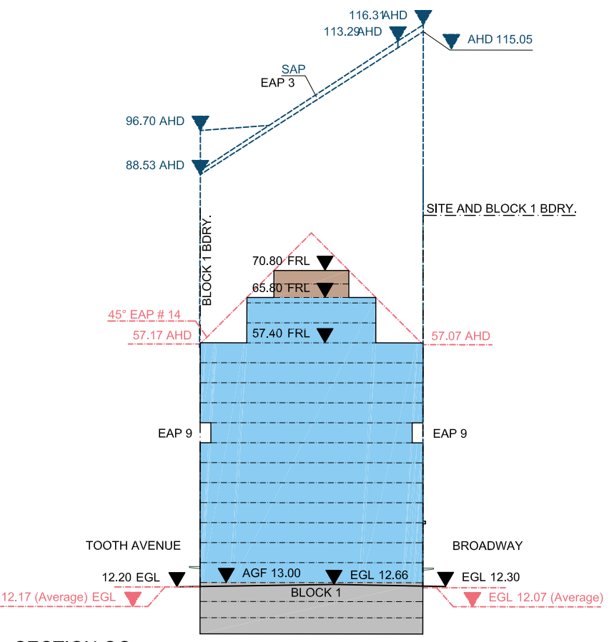
SECTION OO
