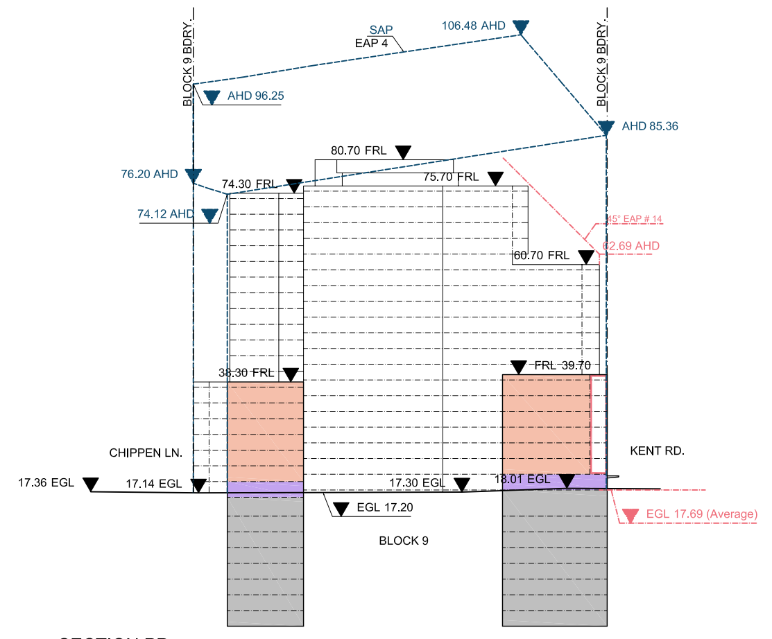
SECTION PP
