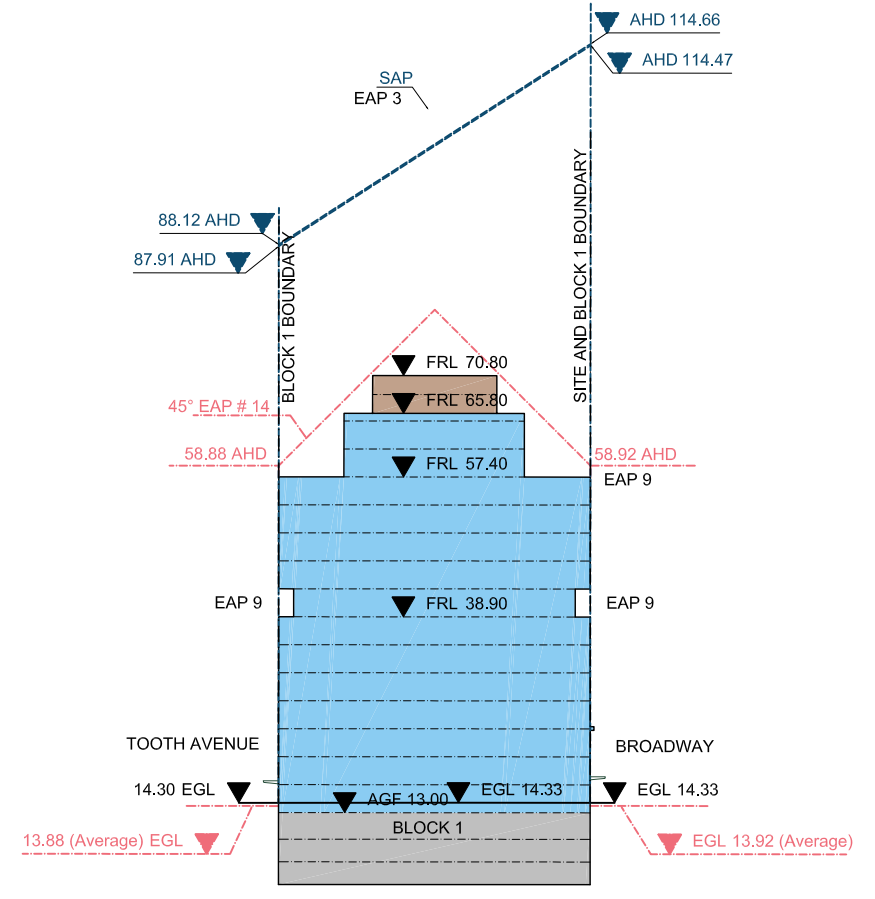
SECTION NN
