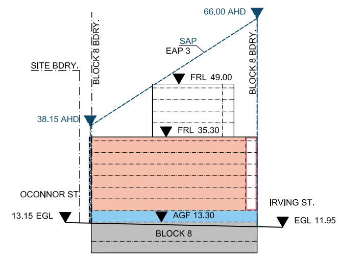
SECTION MM
